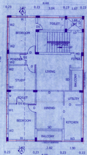
TYPICAL FLOOR PLAN (1st to 4th FLOOR)
